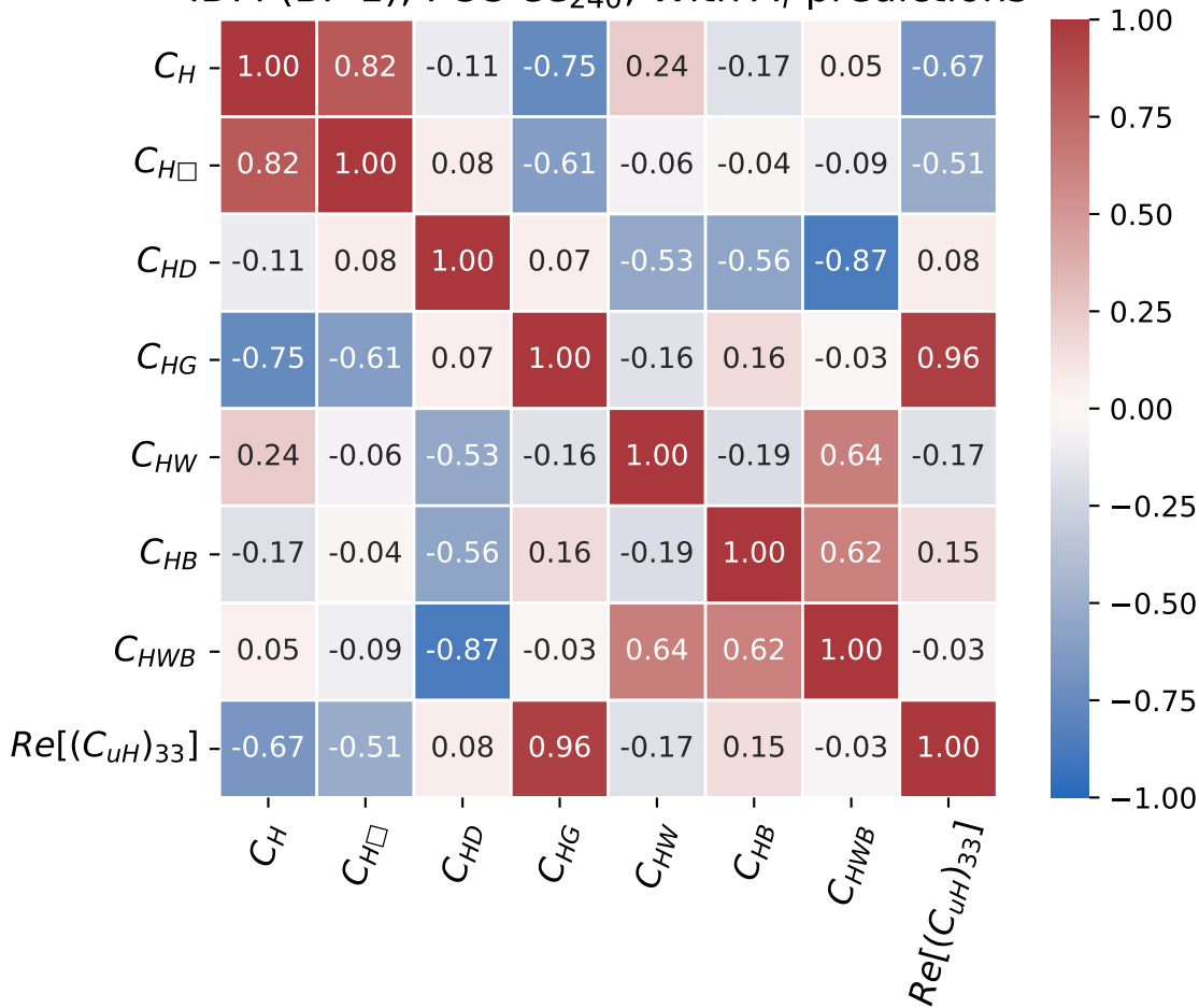
IDM (BP 1), FCC-ee 240 , With A_f predictions
