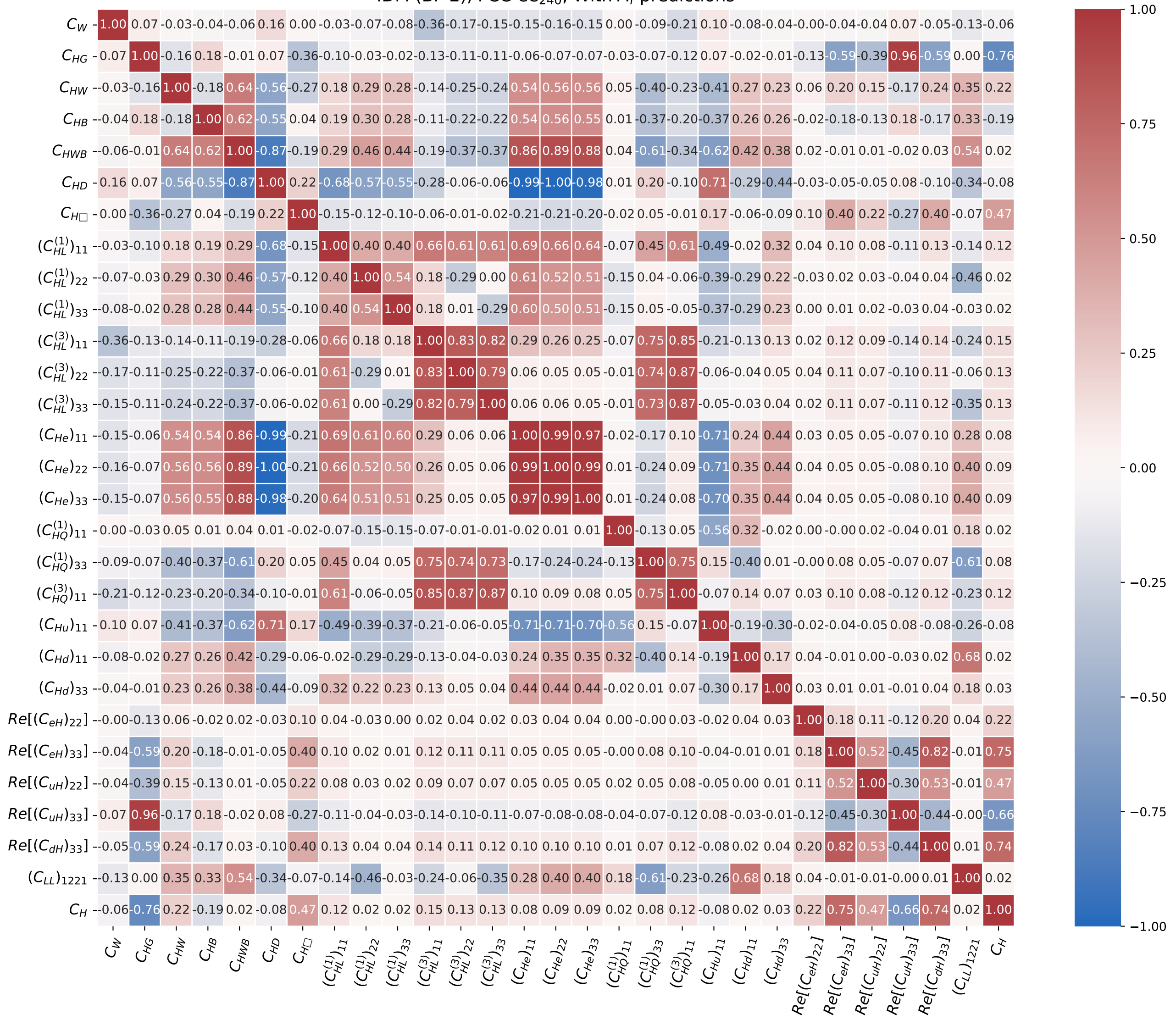
IDM (BP 2), FCC-ee 240 , With A_f predictions
