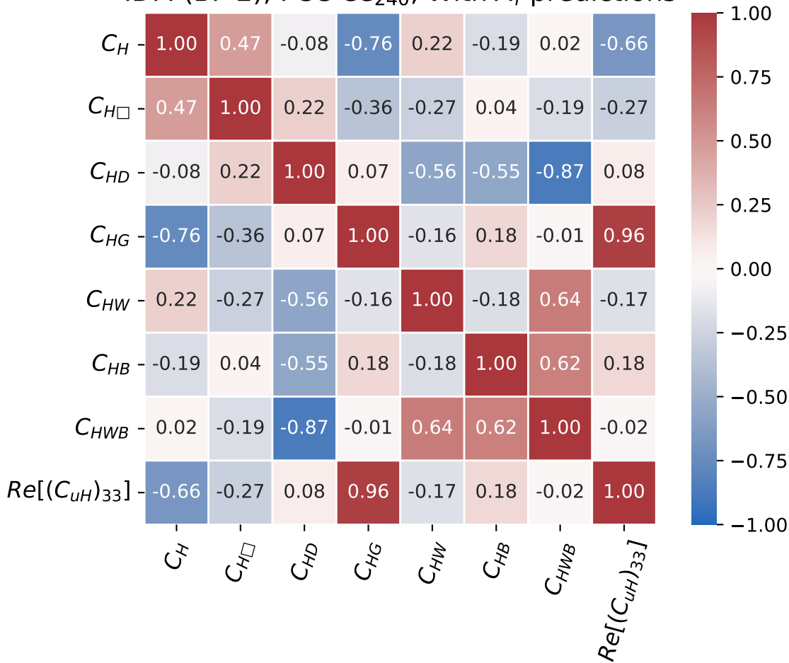
IDM (BP 2), FCC-ee 240 , With A_f predictions
