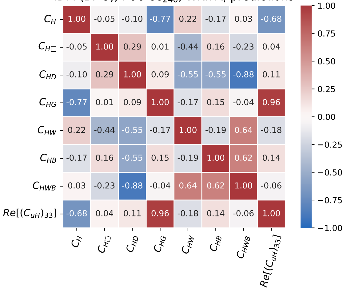
IDM (BP 3), FCC-ee 240 , With A_f predictions
