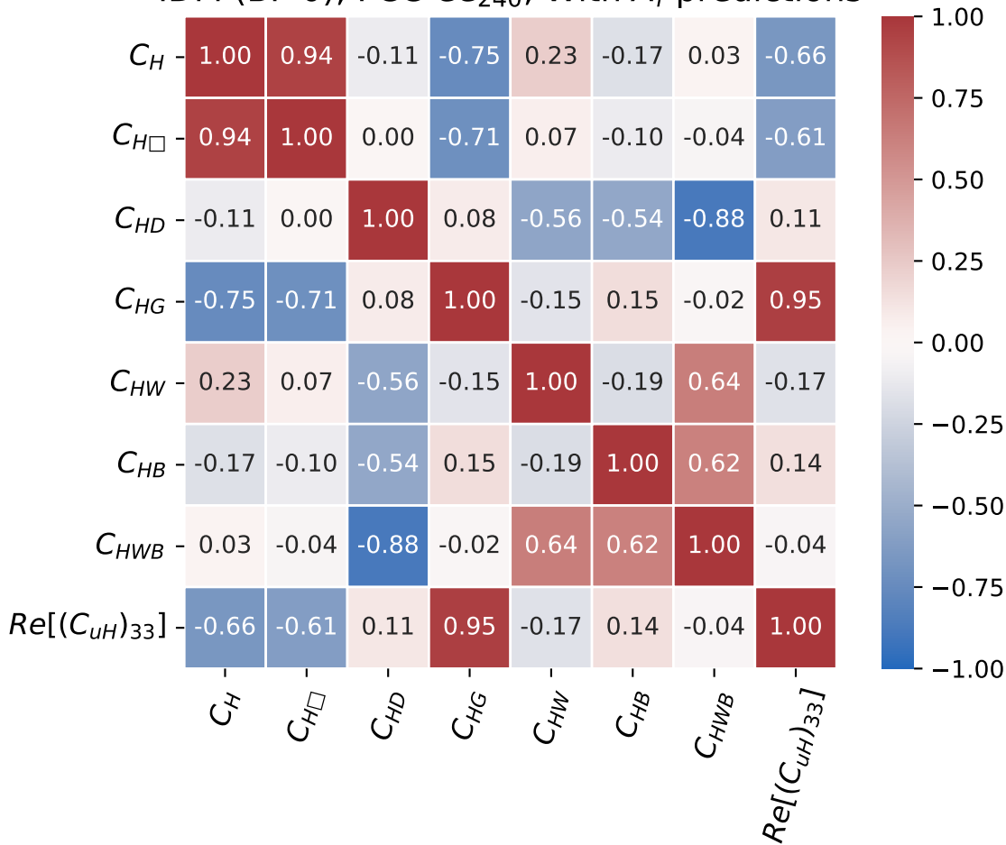
IDM (BP 0), FCC-ee 240 , With A_f predictions
