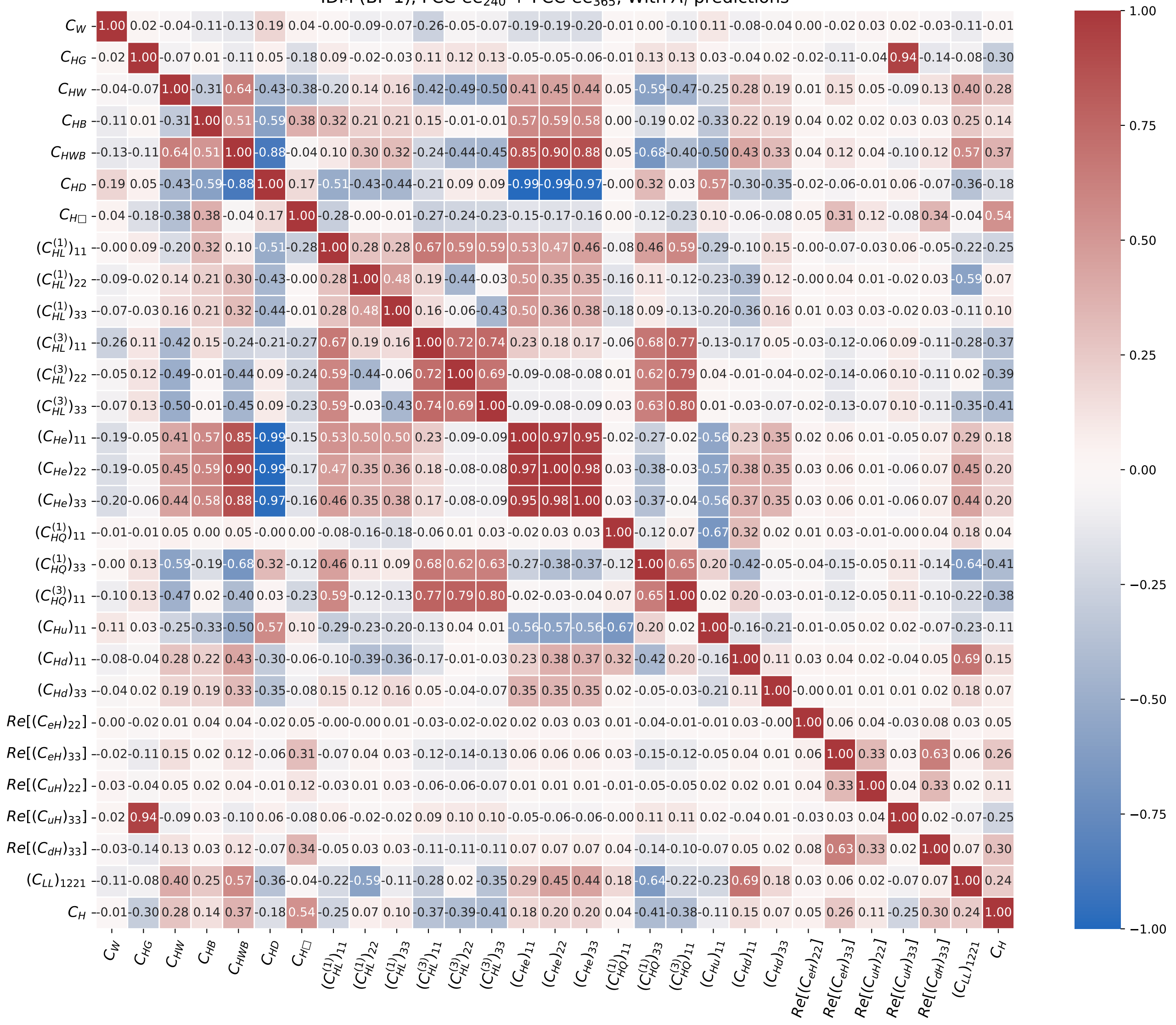
IDM (BP 1), FCC-ee 240 + FCC-ee 365 , With A_f predictions
