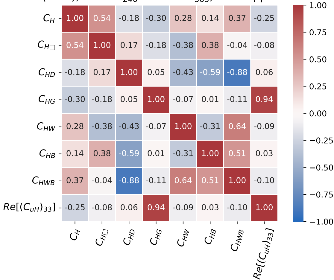
IDM (BP 1), FCC-ee 240 + FCC-ee 365 , With A_f predictions
