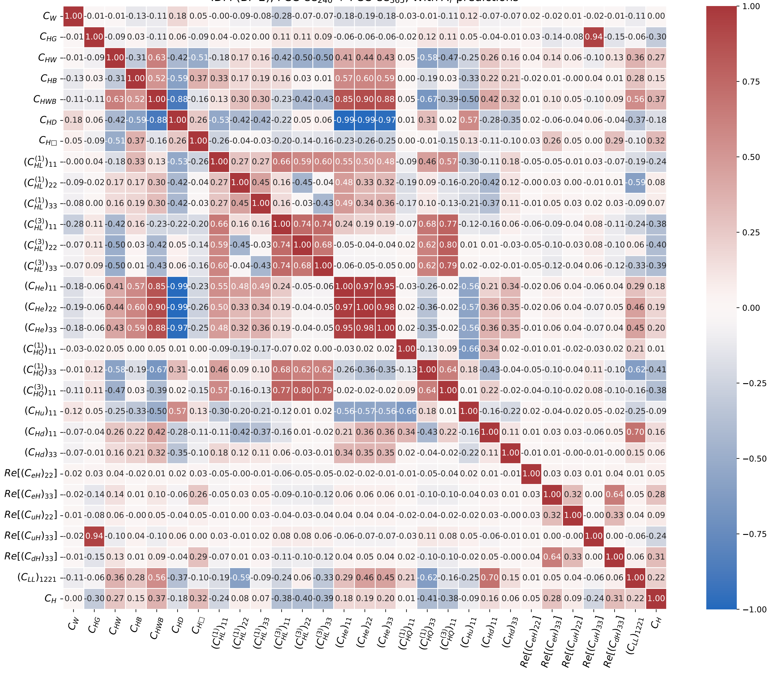
IDM (BP 2), FCC-ee 240 + FCC-ee 365 , With A_f predictions
