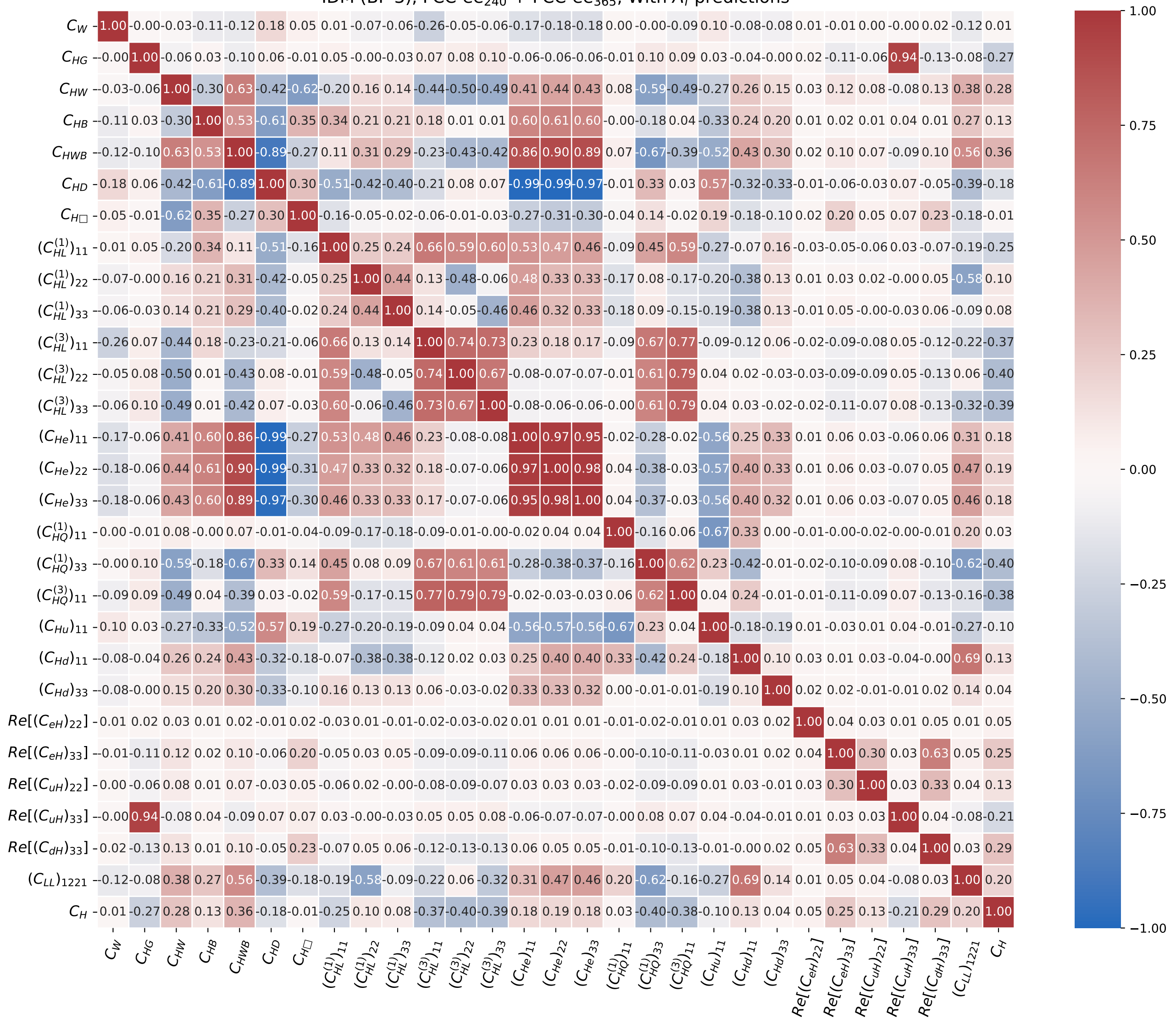
IDM (BP 3), FCC-ee 240 + FCC-ee 365 , With A_f predictions
