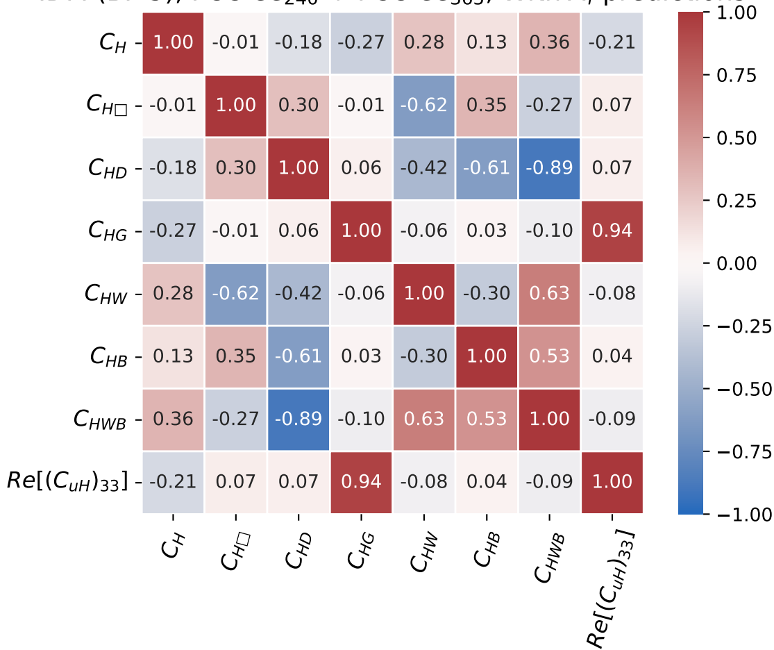
IDM (BP 3), FCC-ee 240 + FCC-ee 365 , With A_f predictions
