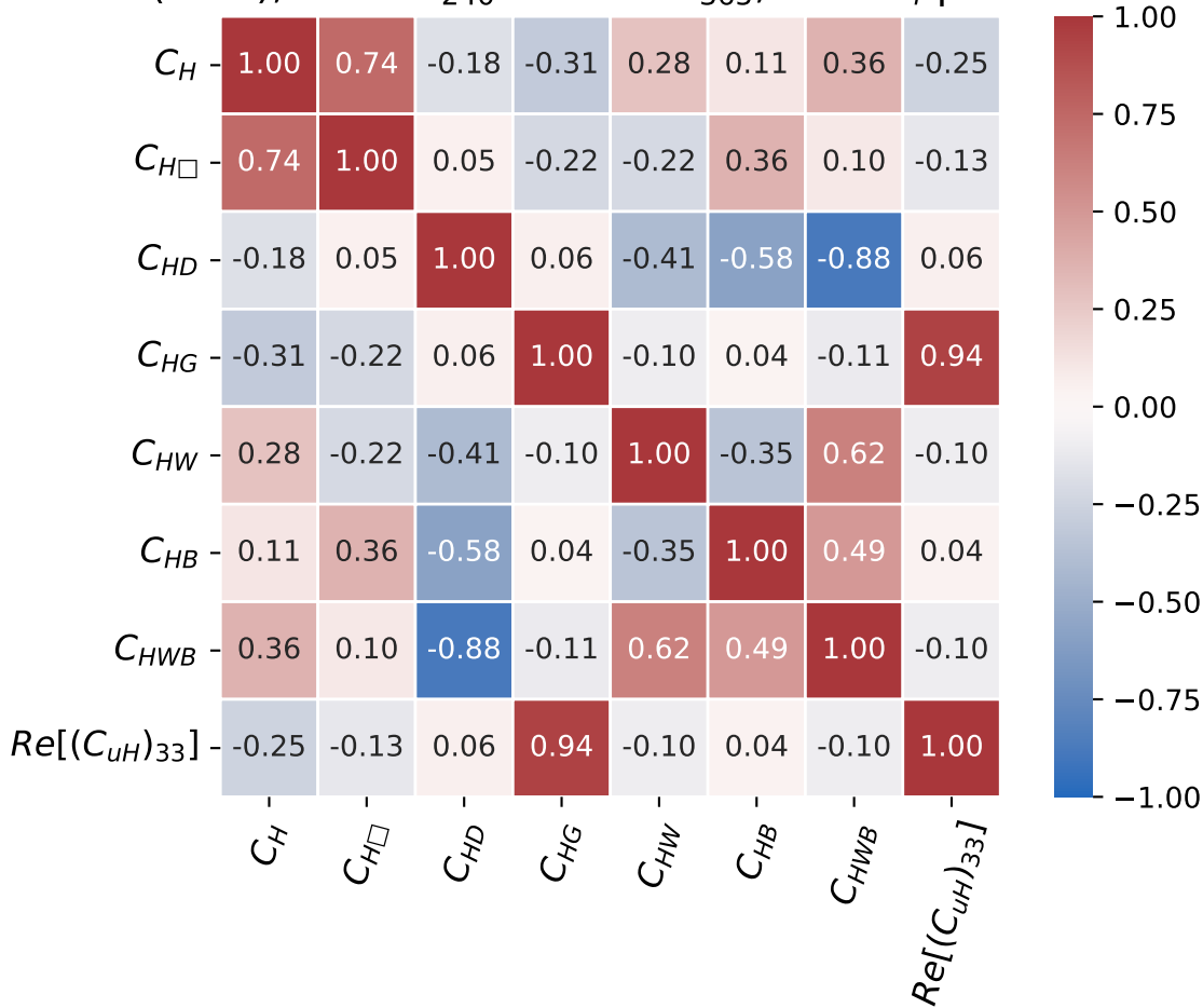
IDM (BP 0), FCC-ee 240 + FCC-ee 365 , With A_f predictions
