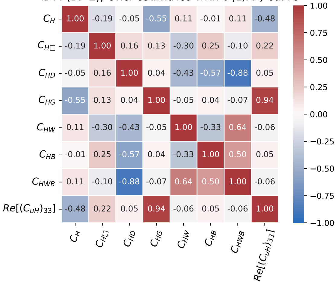
IDM (BP 2), Unc. estimates with \mathcal{O}(1/\Lambda^2) curve
