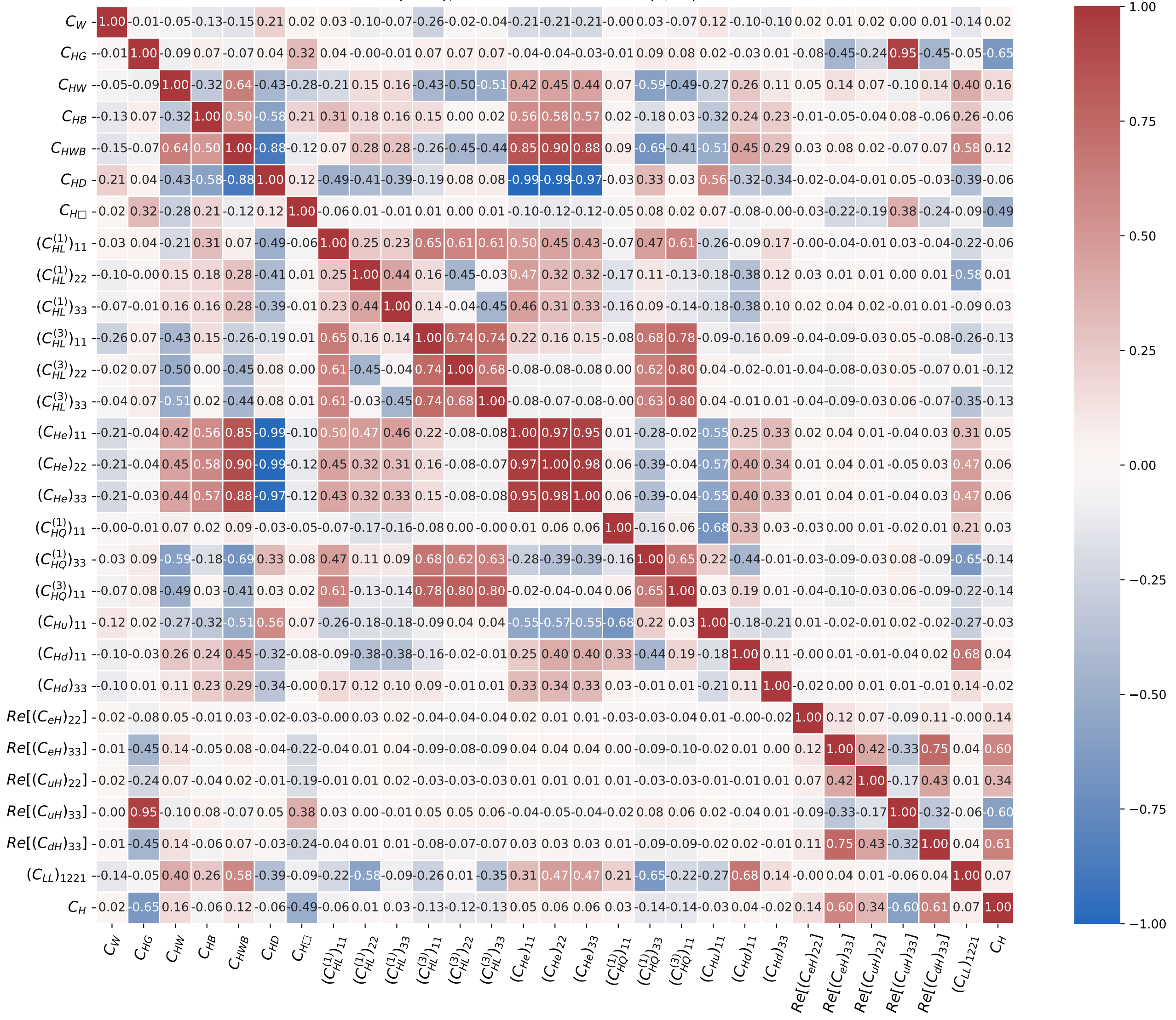
IDM (BP 3), Unc. estimates with \mathcal{O}(1/\Lambda^2) curve
