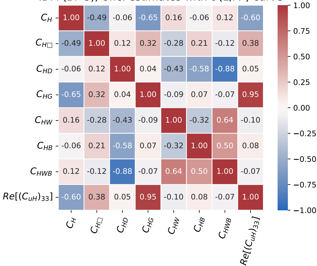
IDM (BP 3), Unc. estimates with \mathcal{O}(1/\Lambda^2) curve
