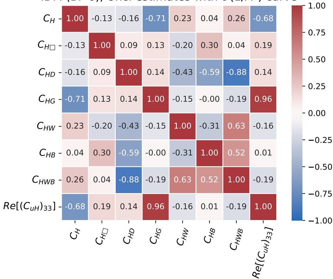
IDM (BP 0), Unc. estimates with \mathcal{O}(1/\Lambda^2) curve
