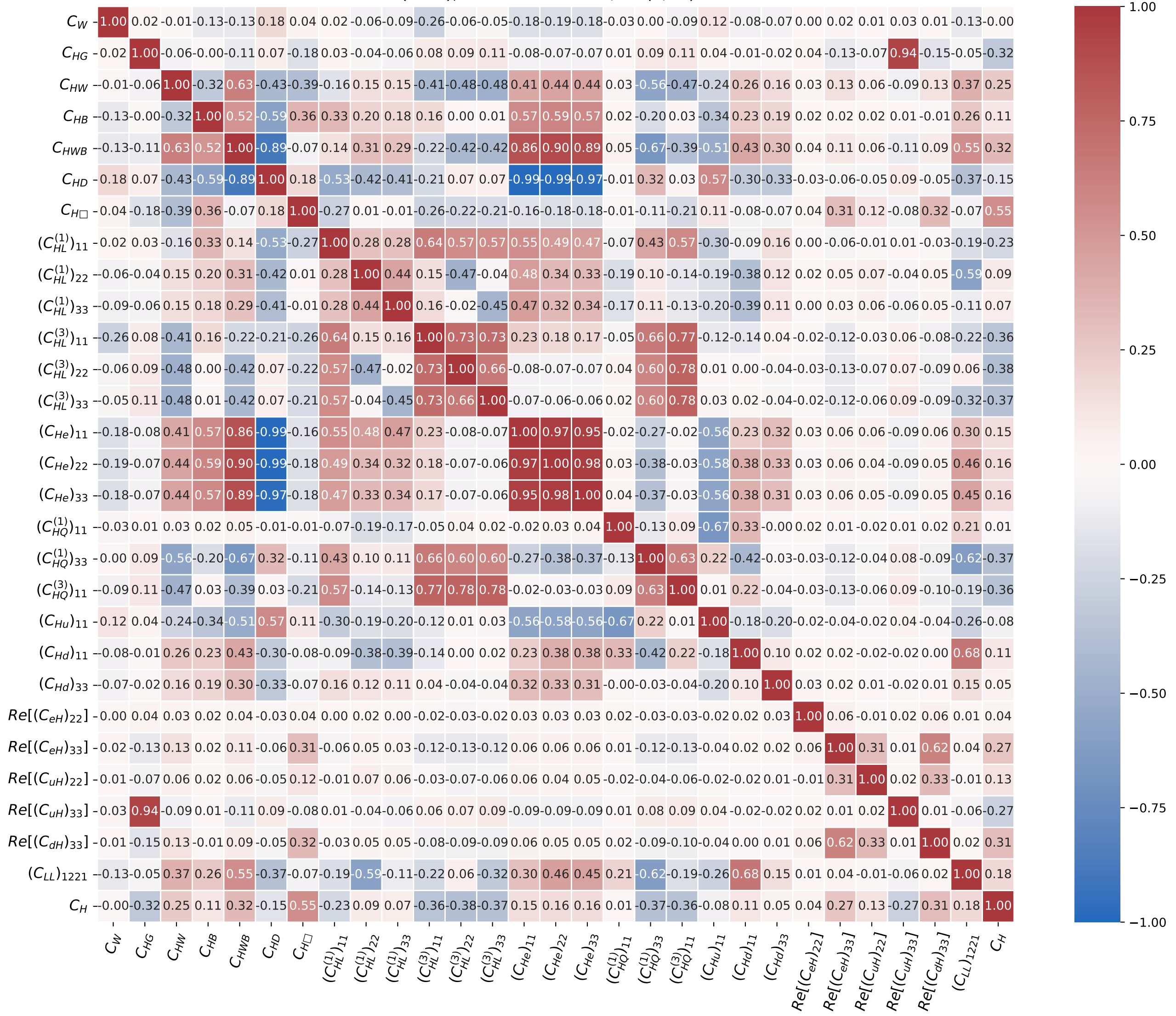
IDM (BP 1), Unc. estimates w/o \mathcal{O}(1/\Lambda^2) curve
