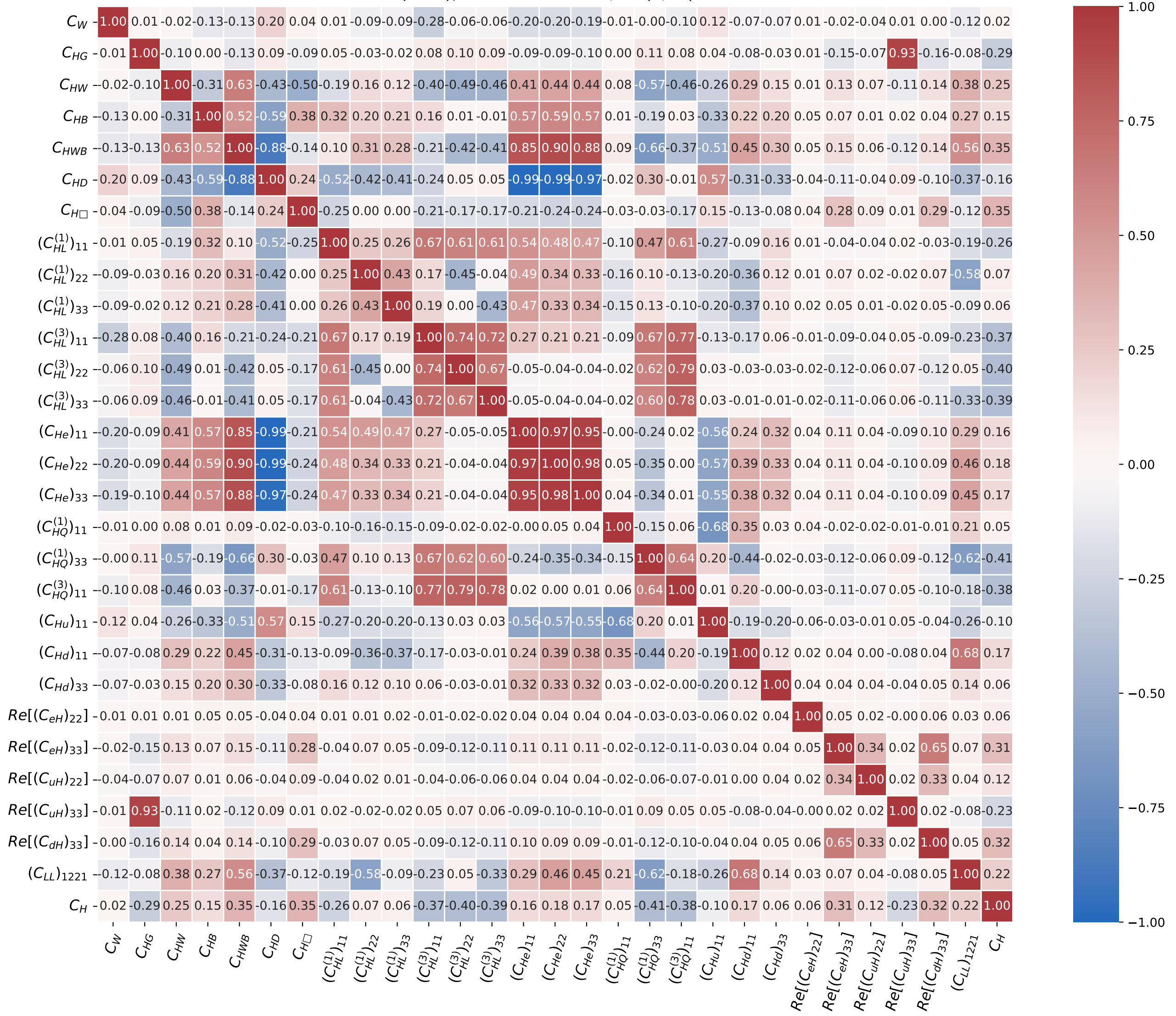
IDM (BP 2), Unc. estimates w/o \mathcal{O}(1/\Lambda^2) curve
