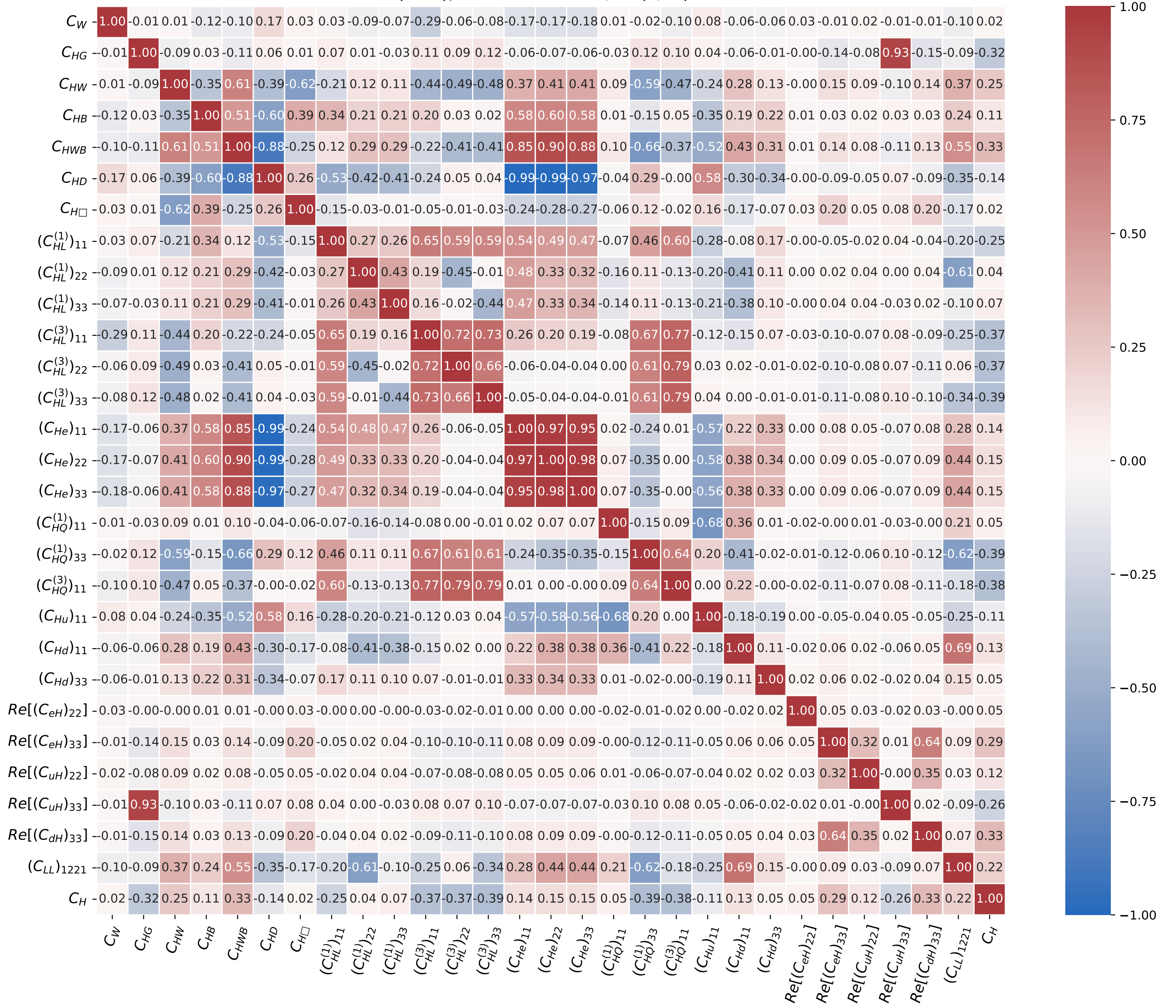
IDM (BP 3), Unc. estimates w/o \mathcal{O}(1/\Lambda^2) curve
