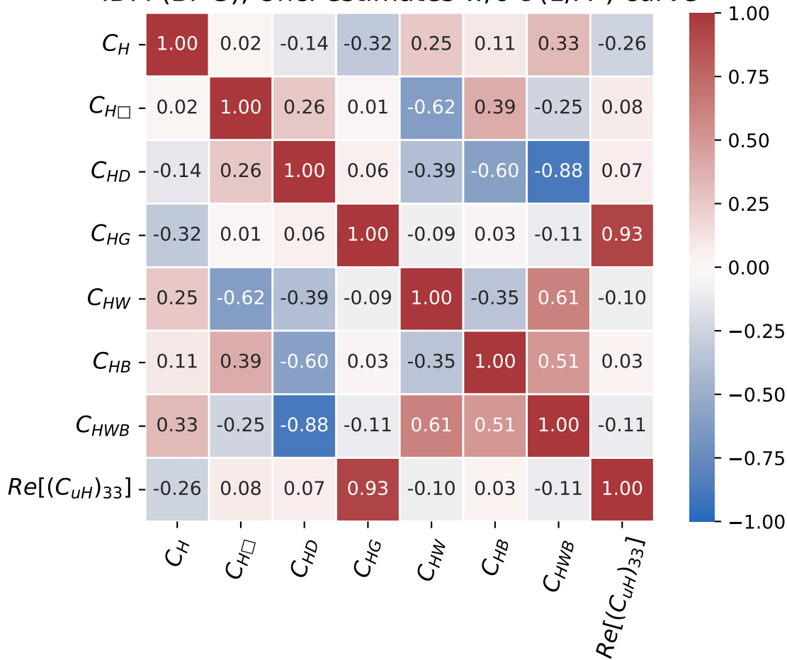
IDM (BP 3), Unc. estimates w/o \mathcal{O}(1/\Lambda^2) curve
