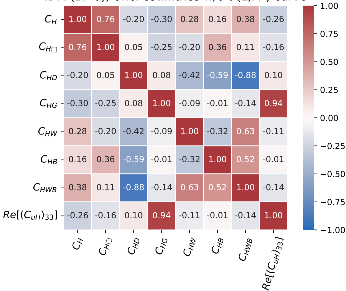
IDM (BP 0), Unc. estimates w/o \mathcal{O}(1/\Lambda^2) curve
