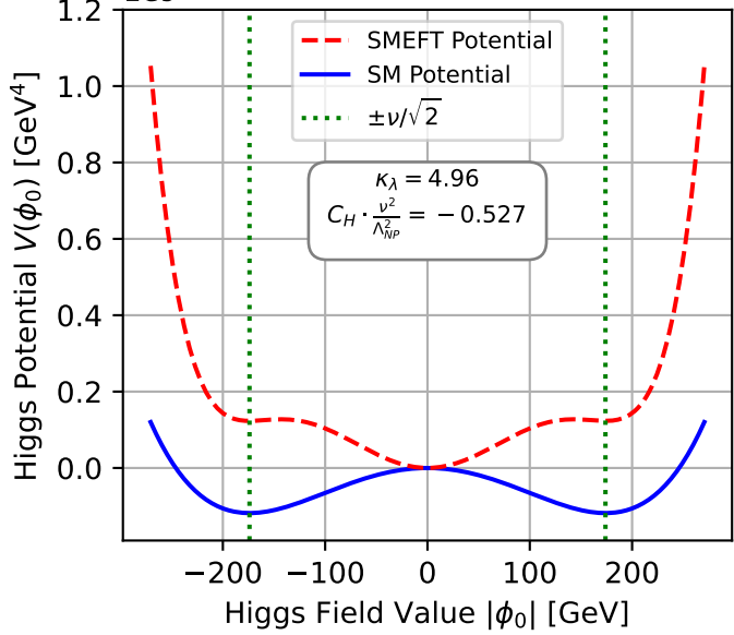
1e9 Higgs Potential in SM and SMEFT
