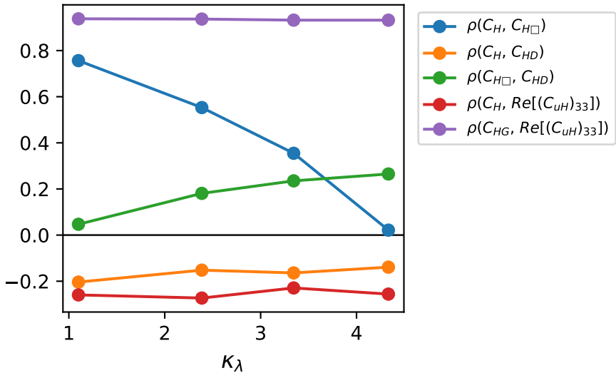
Fitted Wilson coef. correlations
