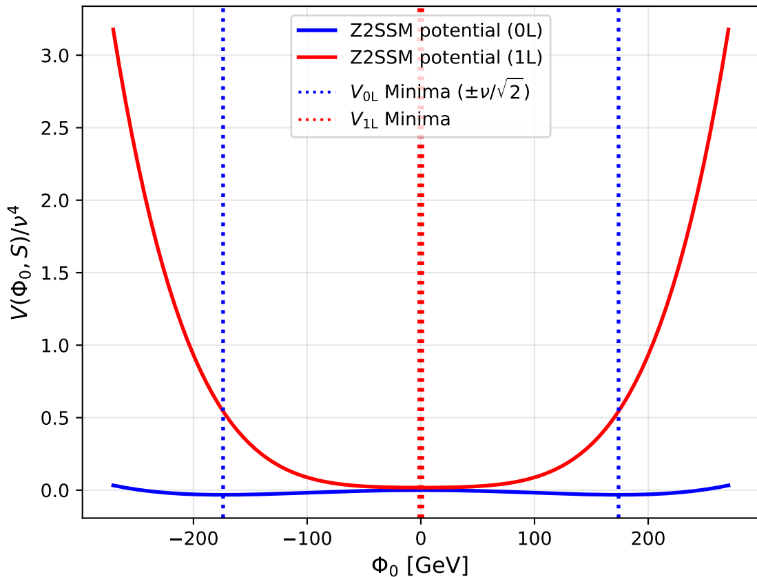
Z2SSM Higgs Potential m_S = 919 GeV, \mu_S = 500 GeV, \lambda_{SH} = 19.6 , \lambda_S = 0.136 , \kappa_\lambda = 3.1
