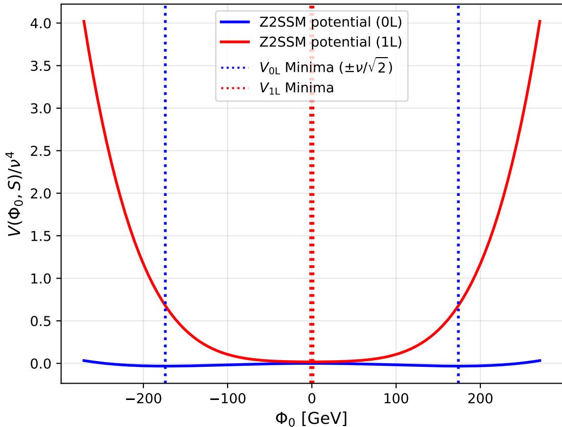
Z2SSM Higgs Potential m_S = 958 \text{ GeV} , \mu_S = 502 \text{ GeV} , \lambda_{SH} = 22 , \lambda_S = 0.458 , \kappa_\lambda = 3.76
