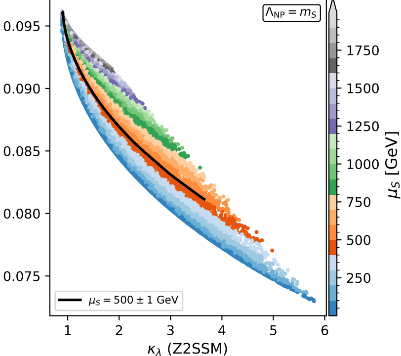
1L Z2SSM vs. 1L SMEFT matching \kappa_\lambda predictions
