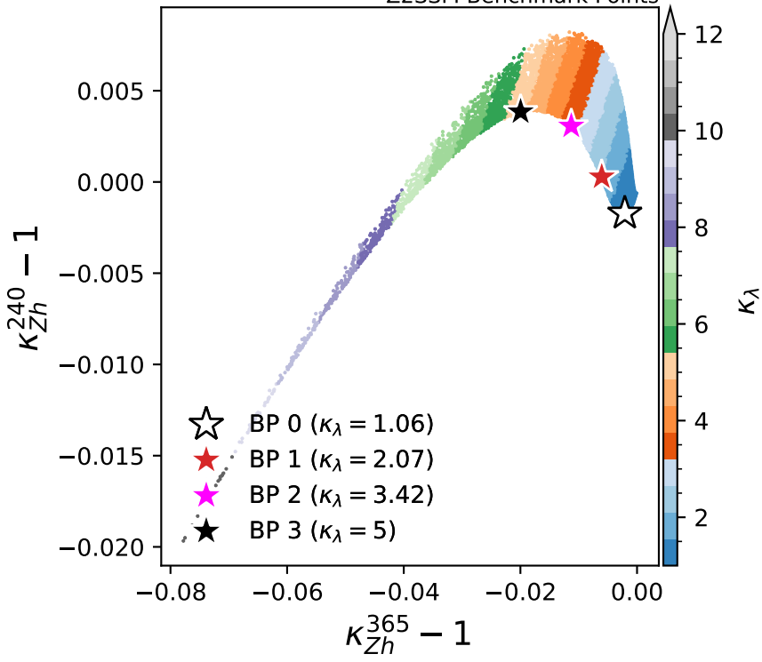
Z2SSM Benchmark Points
