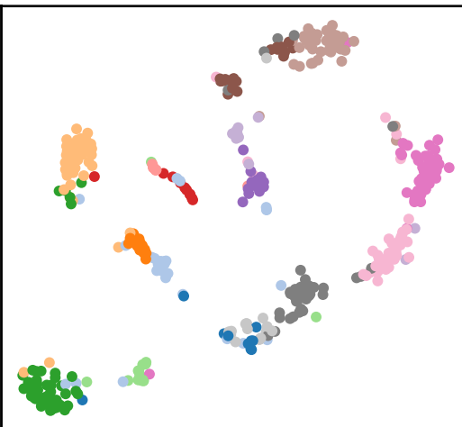
LWM - CLS (Partial Fine-Tuning)
