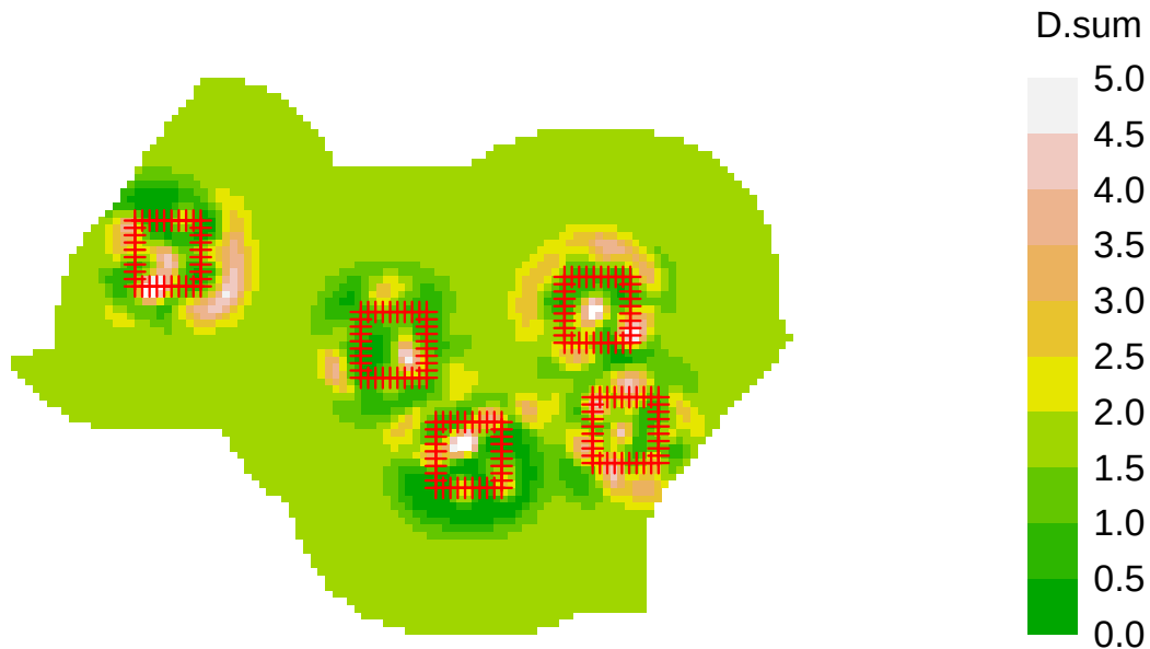
Figure 11.8: Waitarere possum fx surface
