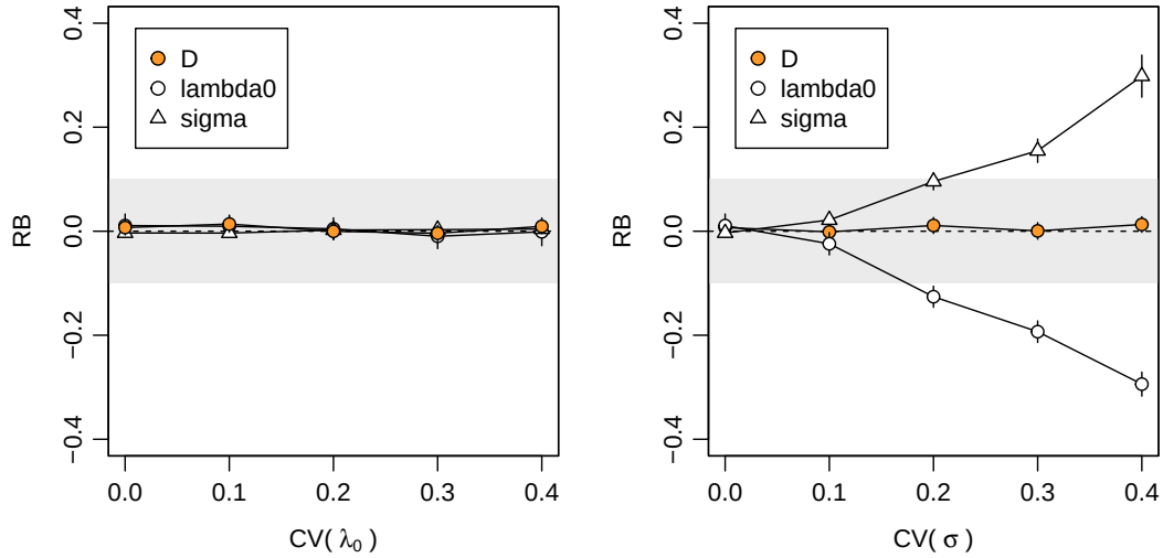
Figure 6.11: Relative bias of parameter estimates from null model given temporal variation in \lambda_0 or \sigma .
