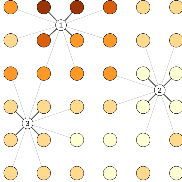
Figure 6.14: Variation in detector efficiency induces individual heterogeneity in overall detection probability p(\vec{x}) . AC 1–3 have similar exposure to detectors but experience respectively high, low and medium detection probability because of the neighbourhoods in which they are located.
