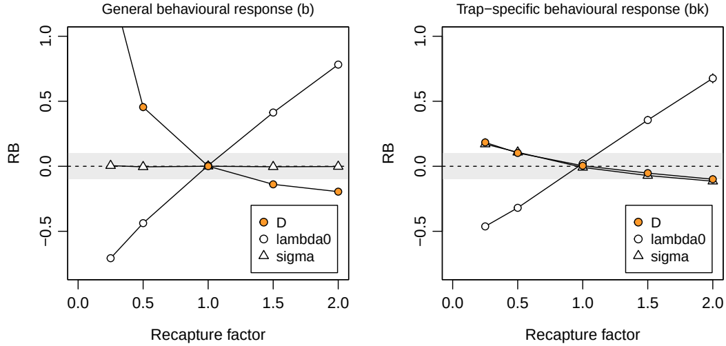
Figure 6.12: Relative bias of parameter estimates from null model given behavioural variation in \lambda_{00} . Relative bias of density was off-scale (+1.41) for recapture factor 0.25 with a general behavioural response.
