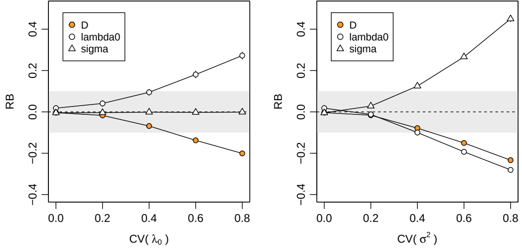
Figure 6.13: Relative bias of parameter estimates from null model given individual variation in \lambda_0 and \sigma^2 .
