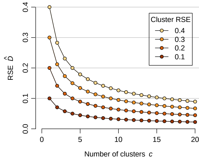
Figure 8.14: Overall \text{RSE}(\hat{D}) from cluster assemblages varying in size and single-cluster RSE.
