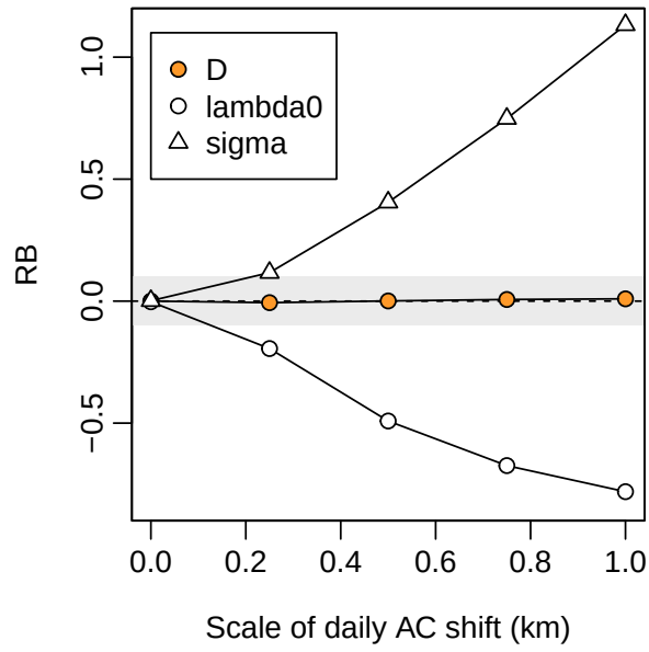
Figure 6.9: Relative bias of density estimates from studies with varying between-occasion movement. Both \hat{\lambda}_0 and \hat{\sigma} are biased by movement, but the net effect on \hat{D} is negligible.
