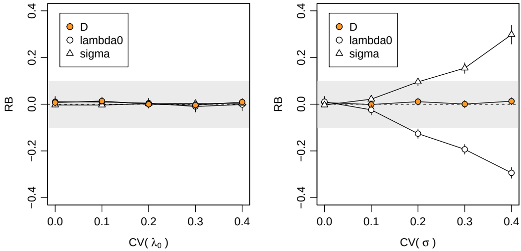
Figure 6.10: Relative bias of parameter estimates from null model given temporal variation in \lambda_0 or \sigma .
