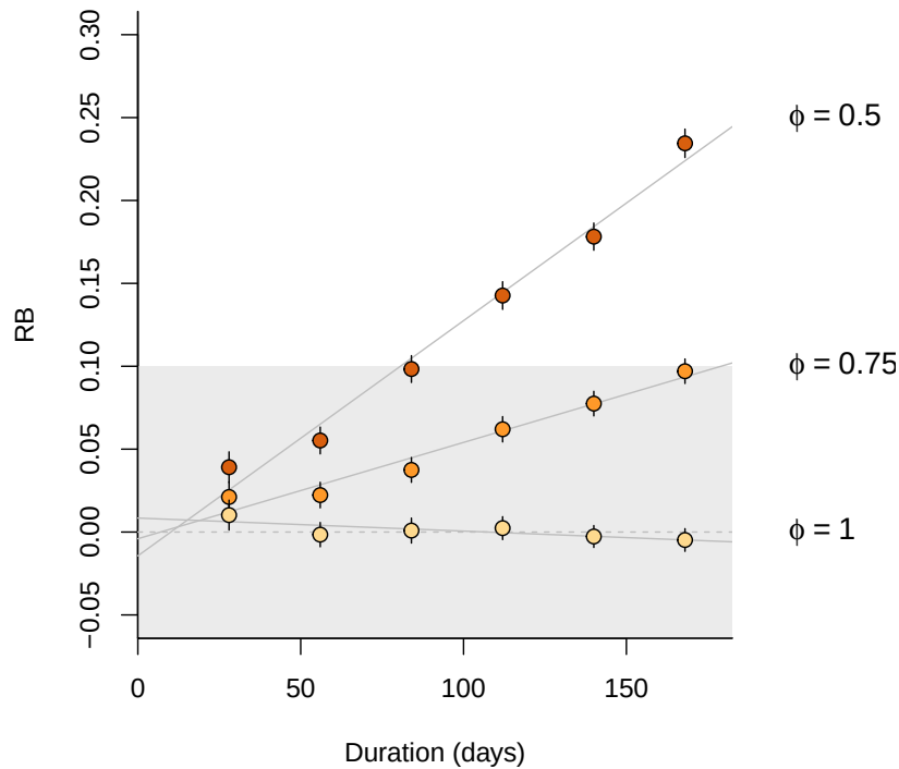
Figure 6.1: Simulated effect of study duration on relative bias of density estimates for three levels of annual survival \phi in a population with constant density. \phi = 1 corresponds to a closed population.
