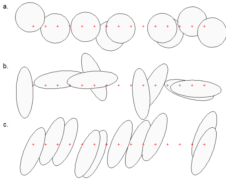
Figure 6.6: SECR models typically assume that home ranges are circular (a). Noncircularity of home ranges causes limited bias in density estimates when ranges are oriented at random with respect to a linear detector array (b). Systematic alignment of ranges to the array (c) causes large bias in \hat{\sigma} and \hat{D} .
