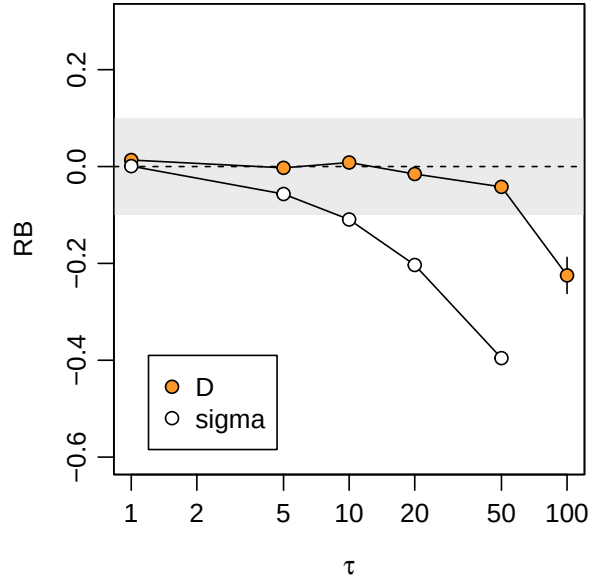
Figure 6.8: Relative bias RB of null-model density estimates of density D and spatial scale \sigma from Ornstein-Uhlenbeck model with autocorrelation parameter \tau .
