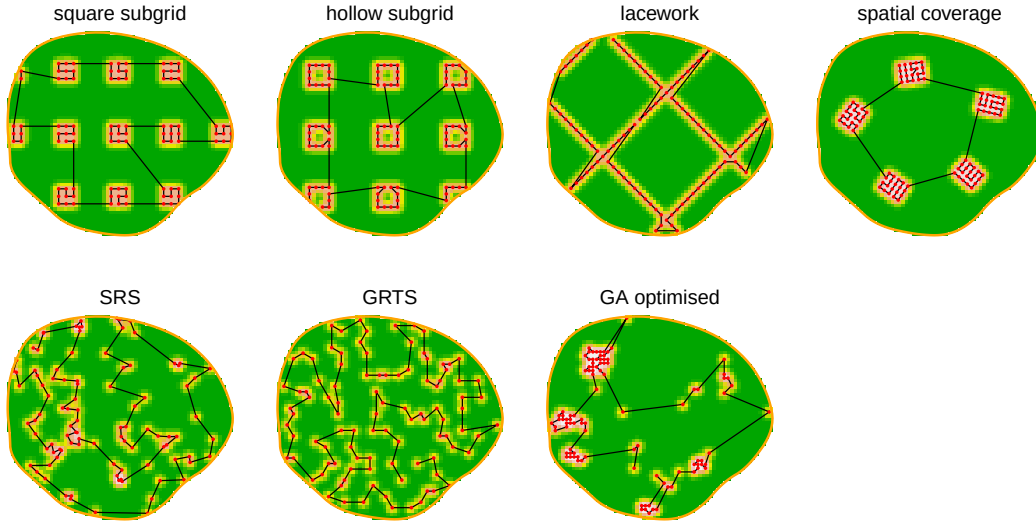
Figure 8.13: Layouts with about 100 detectors in a region 1-km 2 . Colour codes the probability of detection for an individual centred in each pixel (dark green <0.05 , white >0.95 ). Detectors are joined by a minimum-length route.
