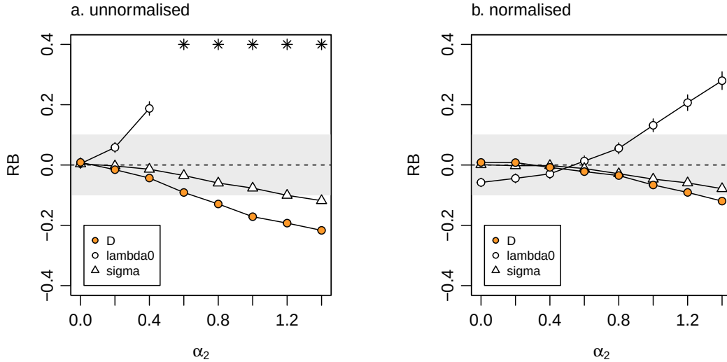
Figure 6.14: Relative bias of parameter estimates from null model when \lambda_0 varies among detectors according to (a) unnormalised model of Royle, Chandler, Sun, et al. (2013), and (b) normalised model of Efford (2014). The magnitude of variation depends on the coefficient \alpha_2 (Eq. 6.1).
