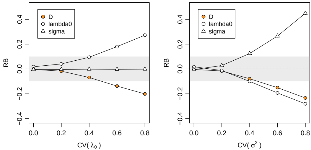
Figure 6.12: Relative bias of parameter estimates from null model given individual variation in \lambda_0 and \sigma^2 .
