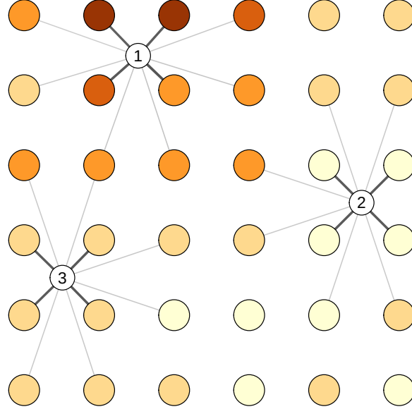
Figure 6.13: Variation in detector efficiency induces individual heterogeneity in overall detection probability p(\vec{x}) . AC 1–3 have similar exposure to detectors but experience respectively high, low and medium detection probability because of the neighbourhoods in which they are located.
