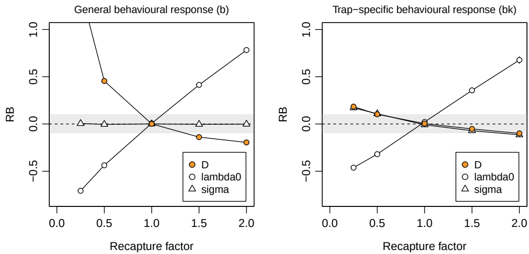
Figure 6.11: Relative bias of parameter estimates from null model given behavioural variation in \lambda_{00} . Relative bias of density was off-scale (+1.41) for recapture factor 0.25 with a general behavioural response.
