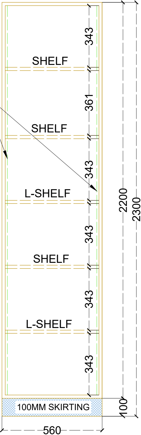
CROCKERY - INTERNAL
