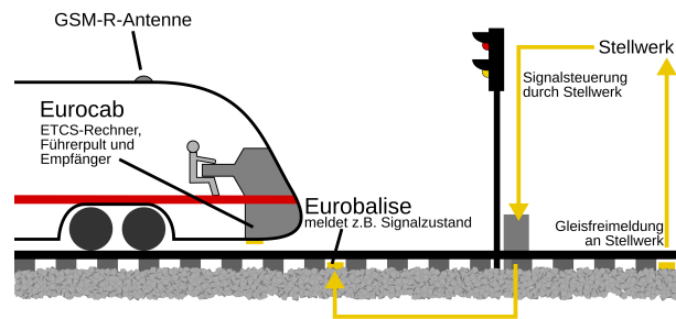
Abb. 2. ETCS Level 1 [SM12]
