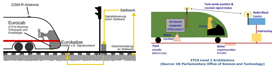
(a) ETCS Level 1 [SM12]
