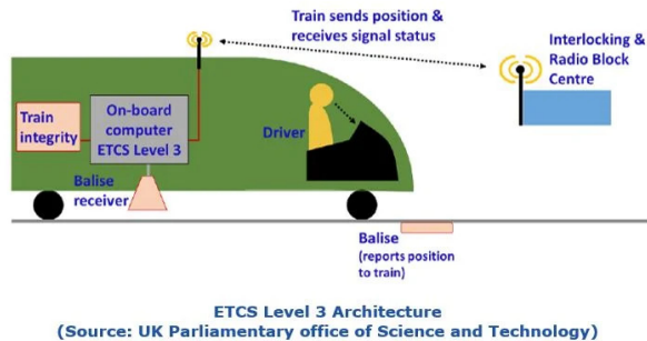
Abb. 4: ETCS Level 3 [ARC]
