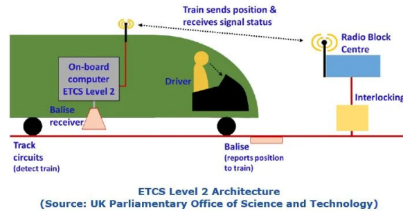
Abb. 3: ETCS Level 2 [ARC]
