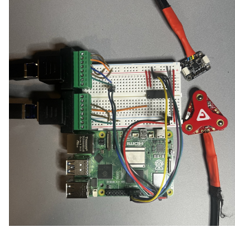
Fig. 1: Data collection device. The Raspberry Pi (bottom) reads, processes, and stores data from the IMU (top right). During data collection, the Pi was powered by a portable battery pack. A box was used to protect the Raspberry Pi from damage, and the IMU was taped to participants’ wrists.
