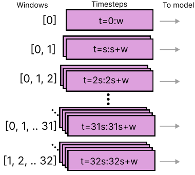
Fig. 7: Real-time inference. Windows of size w = 256 are collected with a stride of s = 64 data points. The most recent T = 32 (or less if not available) windows of data are used to make a prediction. The model makes T predictions, and the prediction for the most recent window is used for real-time inference.
