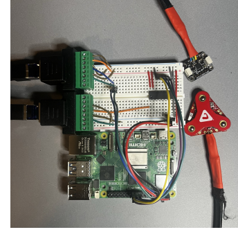
Fig. 1: Data collection device. The Raspberry Pi (bottom) reads, processes, and stores data from the IMU (top right). During data collection, the Pi was powered by a portable battery pack. A box was used to protect the Raspberry Pi from damage, and the IMU was taped to participants’ wrists.
