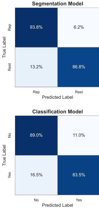
Fig. 9: Confusion Matrices for the segmentation (above) and classification (below) models on the validation sessions. Values are normalized over the true labels (rows). For segmentation, "Rep" represents the time spent during a rep, and "Rest" is the time between reps. The labels for the classification matrix describe whether or not a rep is near-failure ( RiR \leq 2 ).
