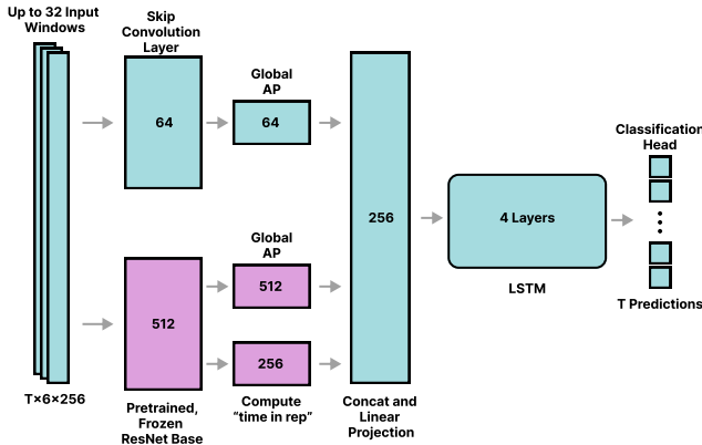
Fig. 6: Classification model architecture.
