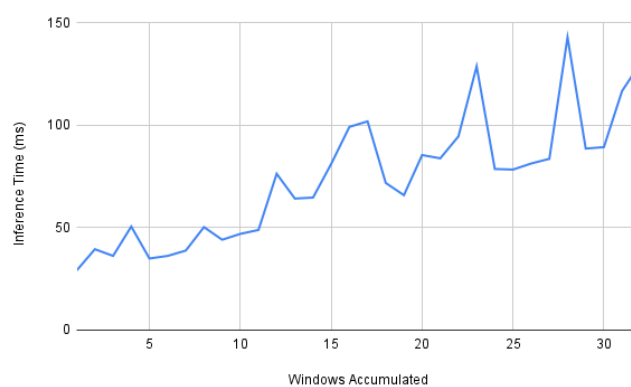
Fig. 12: Deployed model latency on Raspberry Pi. 100 predictions were made in this session, 69 of which were made on a full list of 32 input windows. The average latency of those 69 predictions was used for this figure's last data point.
