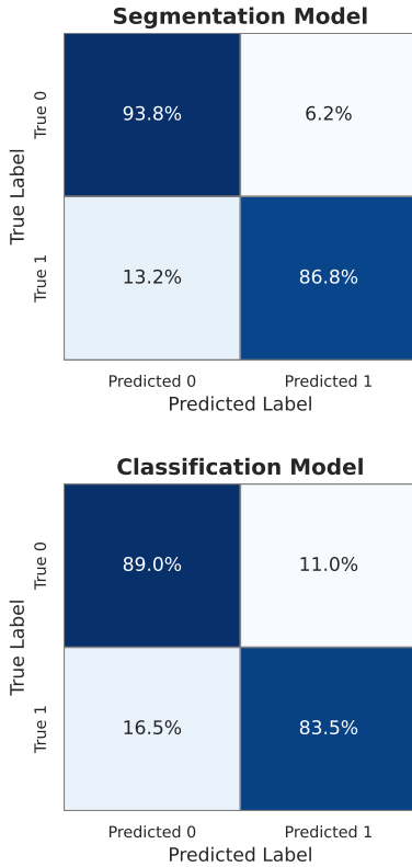
Fig. 8: Confusion Matrices for the segmentation (above) and classification (below) models on the validation sessions. Values are normalized over the true labels (rows).
