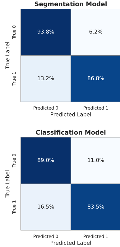
Fig. 8: Confusion Matrices for the segmentation (above) and classification (below) models on the validation sessions. Values are normalized over the true labels (rows).
