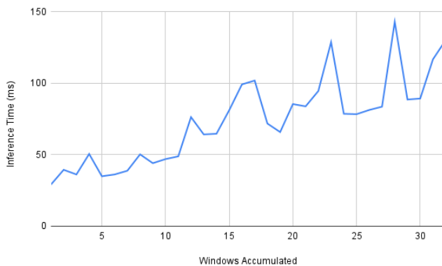
Fig. 10: Deployed model latency on Raspberry Pi. 100 predictions were made in this session, 69 of which were made on a full list of 32 input windows. The average latency of those 69 predictions was used for this figure’s last data point.
