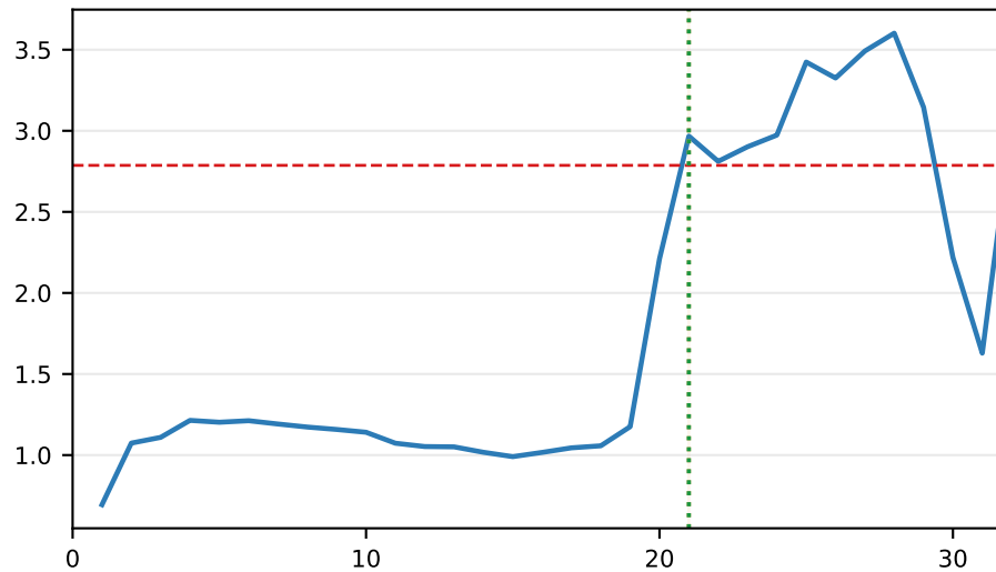
Fanar-1-9B L_kl=L1, L_patch=L32
