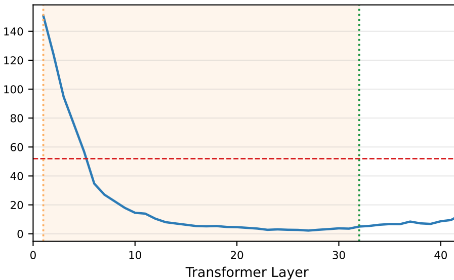
Fanar-1-9B L_kl=L1, L_patch=L32
