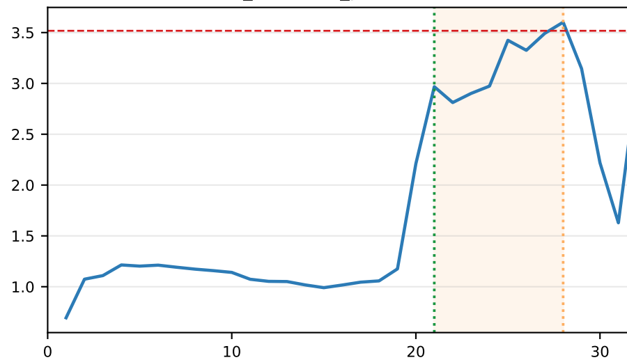
Fanar-1-9B L_kl=L42, L_patch=L32
