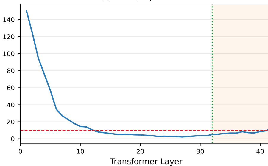
Fanar-1-9B L_kl=L42, L_patch=L32
