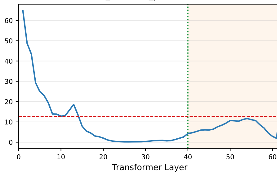
MedGemma-27B-Text-IT L_kl=L62, L_patch=L40
