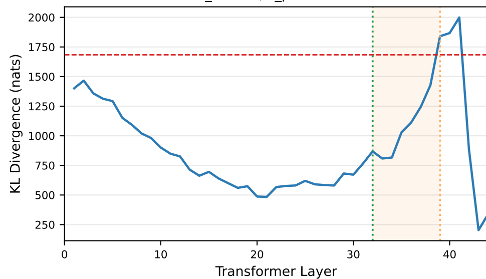
Falcon-H1-7B-Instruct L_kl=L39, L_patch=L32
