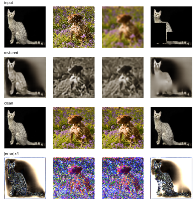
Fig. 9. Task 1 failure cases (worst clean, salt-and-pepper, blur and occlusion test examples).
