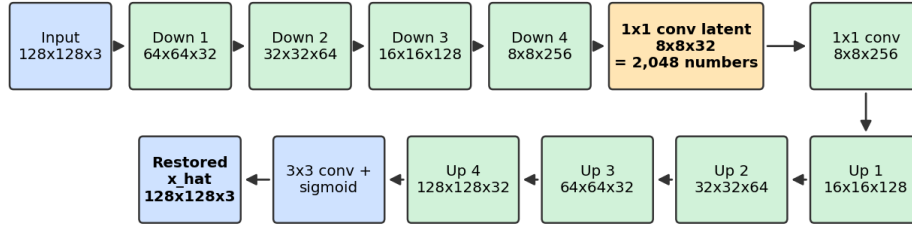
Fig. 2. Architecture of the universal denoising autoencoder (Task 1) and of each Task 2 specialist for the selected configuration ( c = 32 , spatial latent 8 \times 8 \times 32 ): four stride-2 encoder stages, a 1 \times 1 -convolutional bottleneck of 2,048 numbers, four transposed-convolution decoder stages, and no skip connections.
