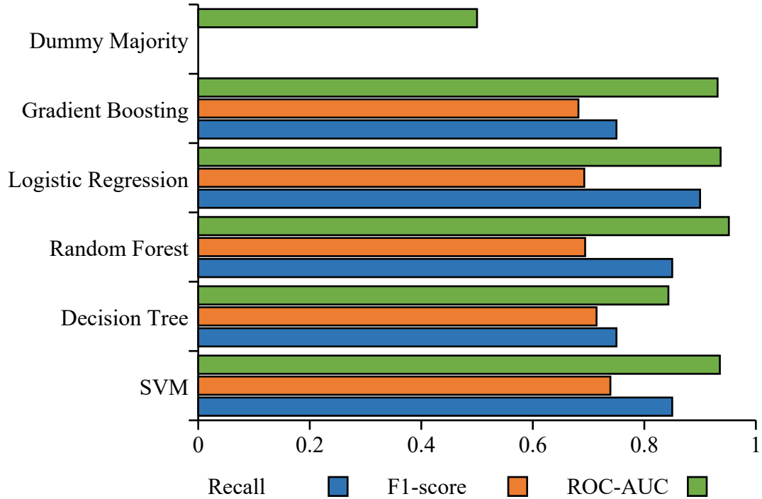
Figure 2. Performance-Aware Model Comparison
