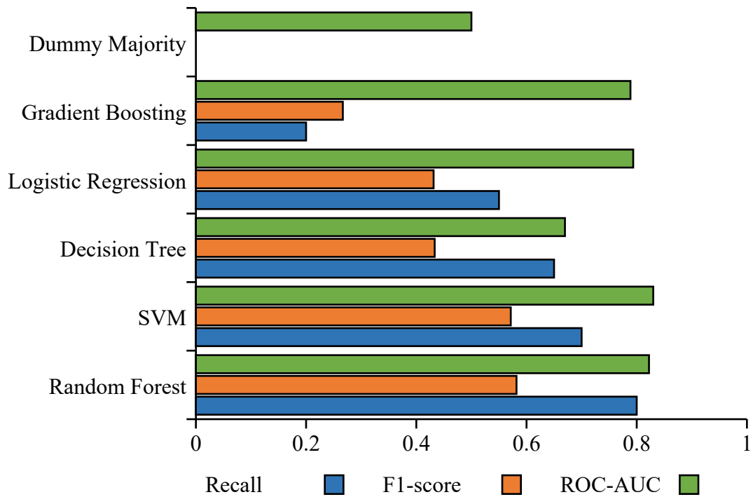
Figure 1. Early-Warning Model Comparison
