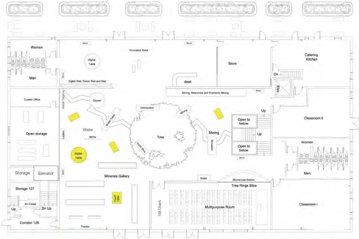
1 Building Plan: First Floor Scale: 1/16" = 1'-0"
