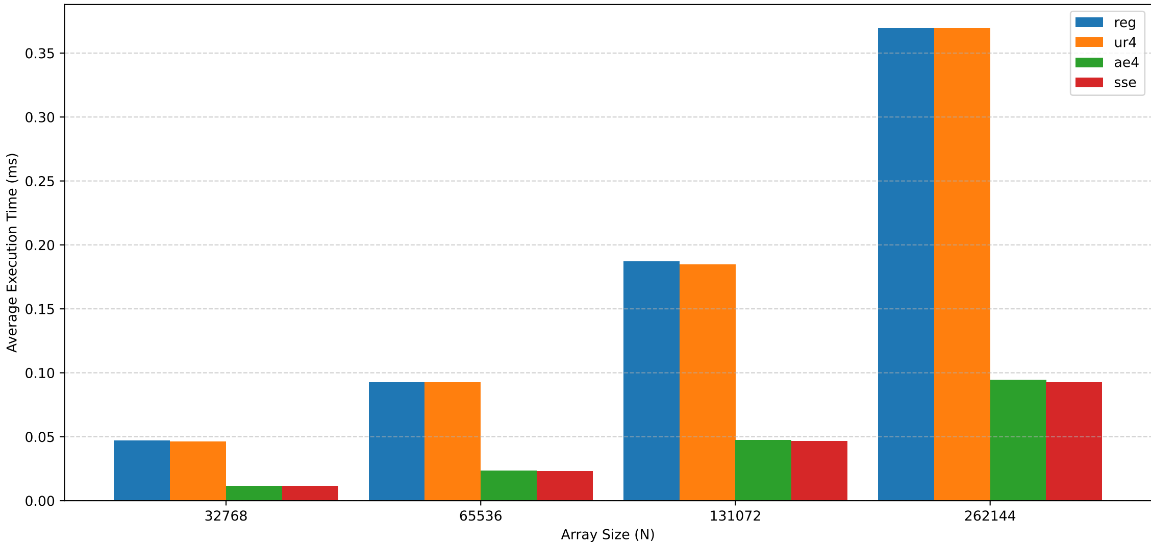
Dot Product Performance Comparison
