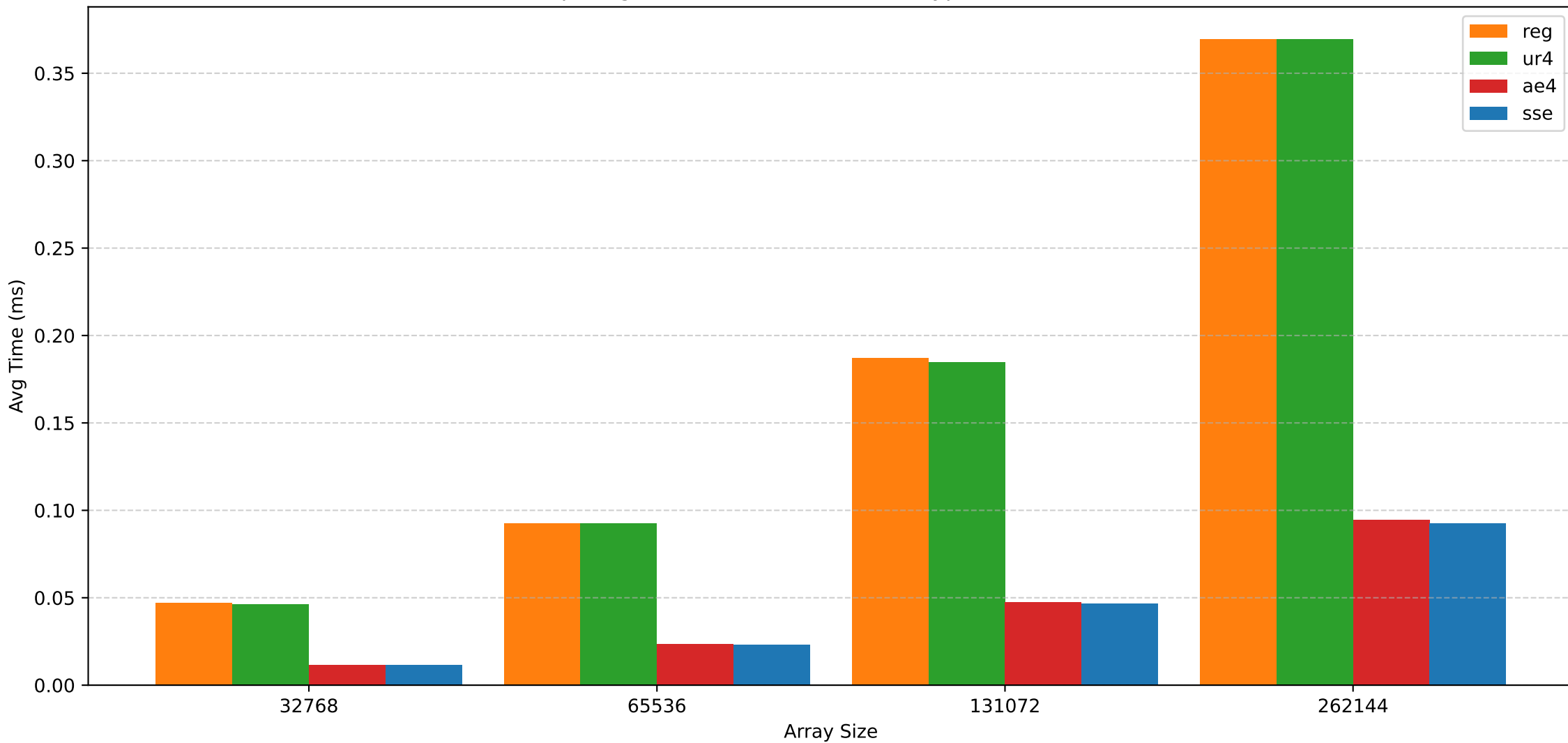
Comparing Performance of Different Types of Dot Product
