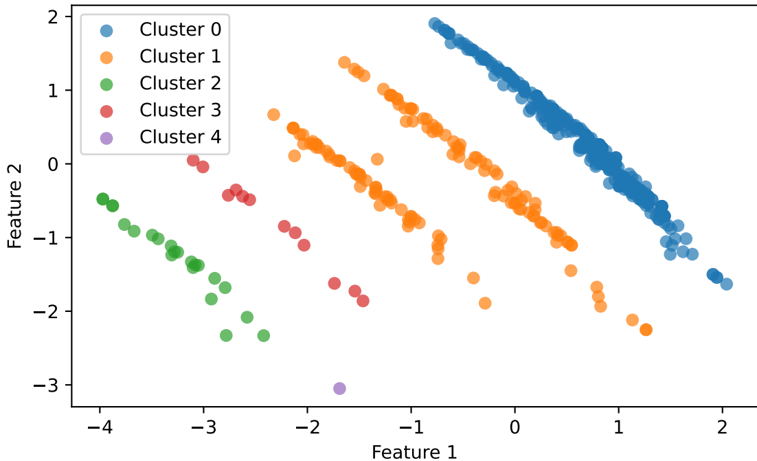
Robust Standardize DBSCAN
