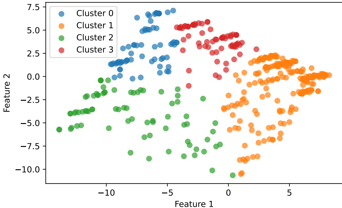
Original Data KMeans Results
